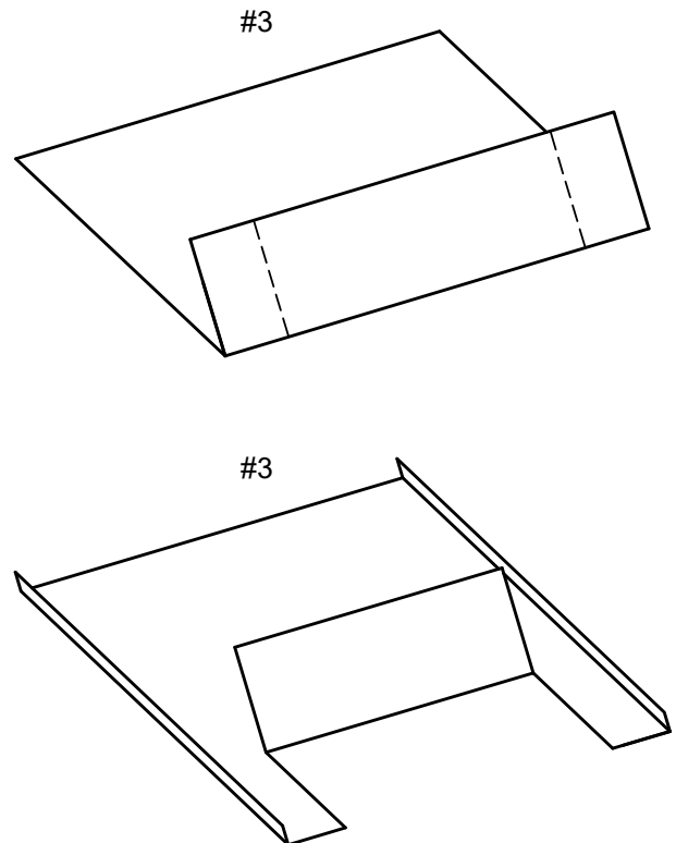
#3 is the Pan flashing. Order the proper size for the curb height of your skylight, 5-1/2" (ELP5) or 3-1/2" (ELP3).
