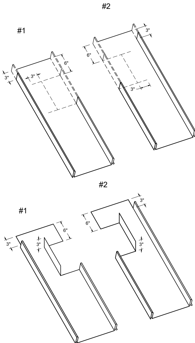
Parts shown after they have been cut and bent.
